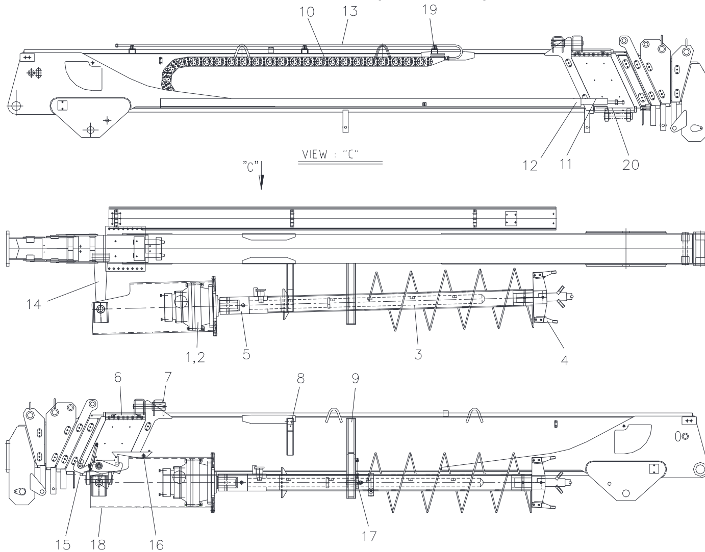
Fig. 13 SCS876 AUGER BOOM ASS'Y (W42000)
