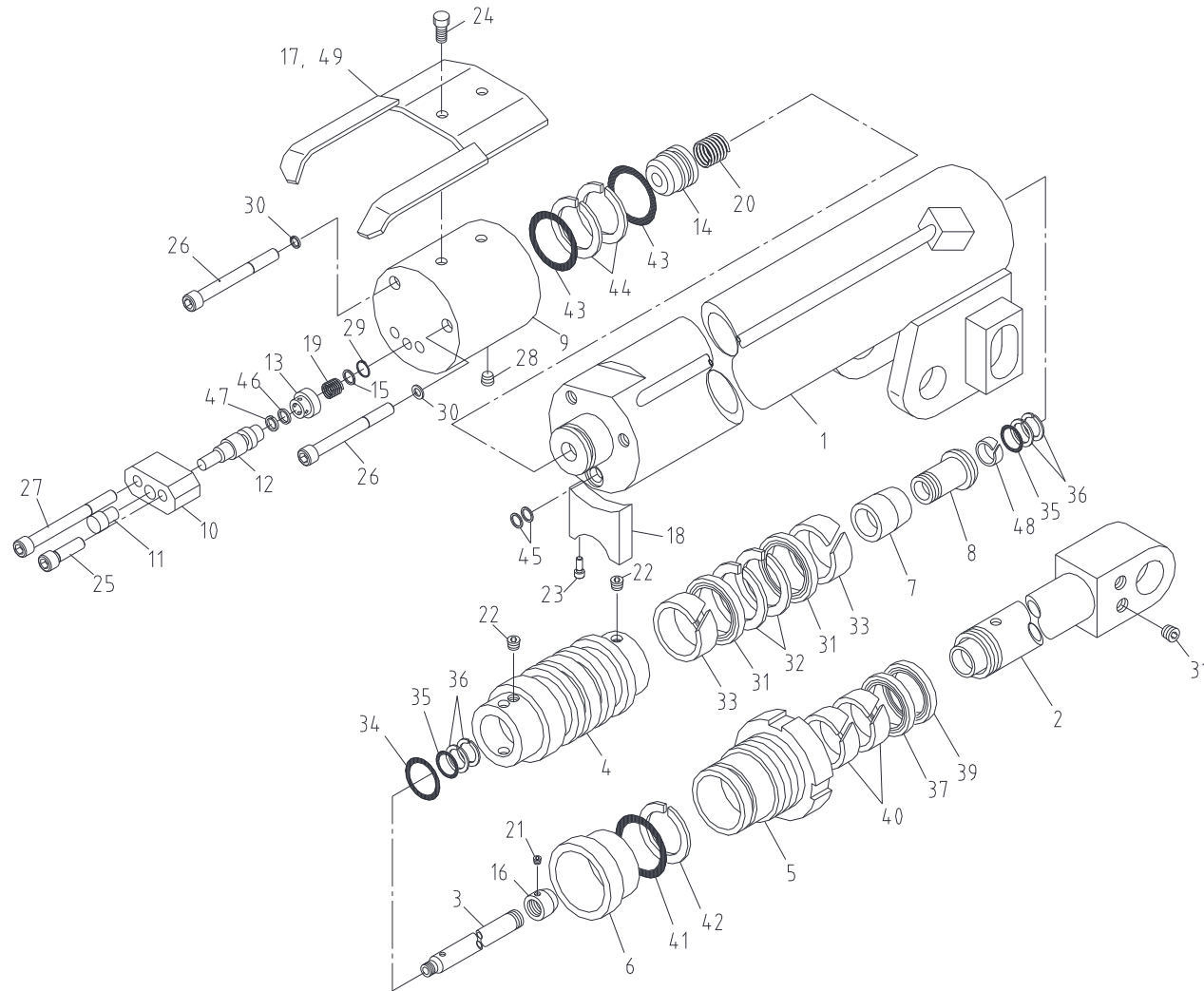
Fig. 1-1-1 SCS876 TELESCOPIC CYL'(1st) ASS'Y
