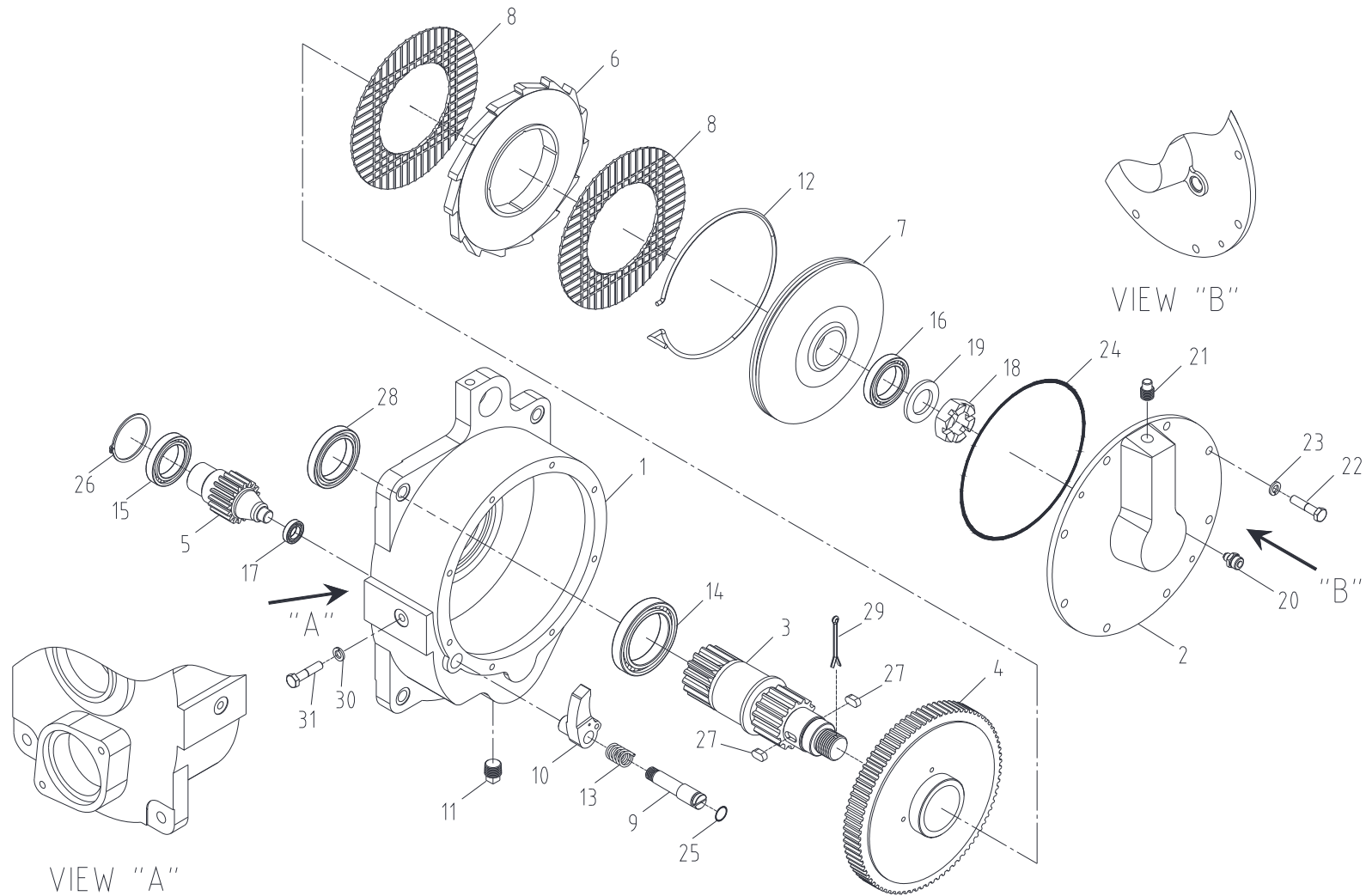
Fig. 2-1 SCS876 WINCH R/ G ASS'Y
