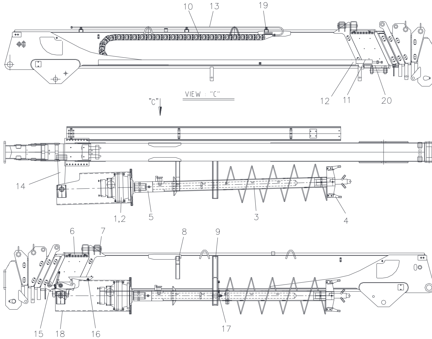
Fig. 12 SCS876 AUGER BOOM ASS'Y (W43000)
