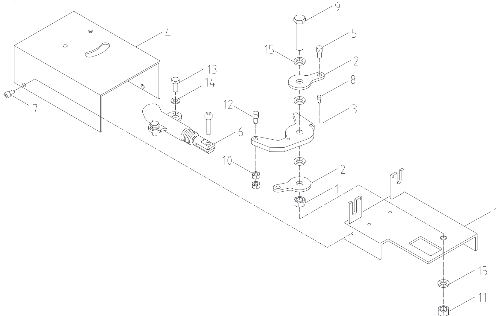
Fig. 9-3 SCS876 ACC'L SYSTEM PART
